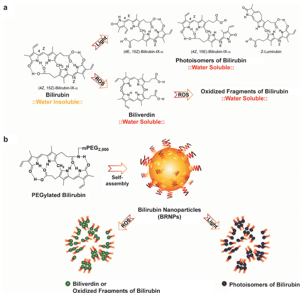
Scheme 1. A) The solubility switch of bilirubin. b) A schematic representation of disruption of the BRNPs in response to light or ROS stimuli.
