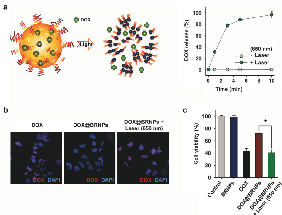
Figure 2. DOX@BRNPs as light-responsive nanoparticles that can be used in antitumor phototherapy. a) DOX release from the DOX@BRNPs in the absence and presence of \lambda = 650 nm laser irradiation ( 90 \text{ mWcm}^{-2} , 10 min). Data are presented as the mean \pm SD ( n = 5 ). b) A confocal fluorescence image of A549 cells treated with culture medium, free DOX ( 10 \mu\text{M} ), the BRNPs ( 10 \mu\text{M} ), the DOX@BRNPs ( 10 \mu\text{M} DOX; 10 \mu\text{M} BRNPs), or the DOX@BRNPs for 4 h with \lambda = 650 nm laser irradiation ( 90 \text{ mWcm}^{-2} , 5 min). DOX (red) and nuclei (blue) were visualized. c) Cell viability of A549 cells incubated with culture medium (control), DOX ( 10 \mu\text{M} ), the BRNPs ( 10 \mu\text{M} ), the DOX@BRNPs ( 10 \mu\text{M} DOX; 10 \mu\text{M} BRNPs), or the DOX@BRNPs for 4 h with \lambda = 650 nm laser irradiation ( 90 \text{ mWcm}^{-2} , 5 min). Data are presented as the mean \pm SEM. ( n = 6 ; *p < 0.001 , one-way ANOVA).
